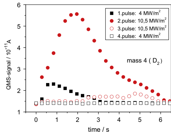
Fig. 4. Desorption of mass 4 (deuterium) occurred during all pulses applied on tile 13. It reveals that the dominant amount of gas is desorbed during the first 10.5 \text{ MW/m}^2 pulse at temperatures of about 700 \text{ °C} (compare with Fig 3). The background signal is 1.4 \cdot 10^{-11} \text{ A} .
