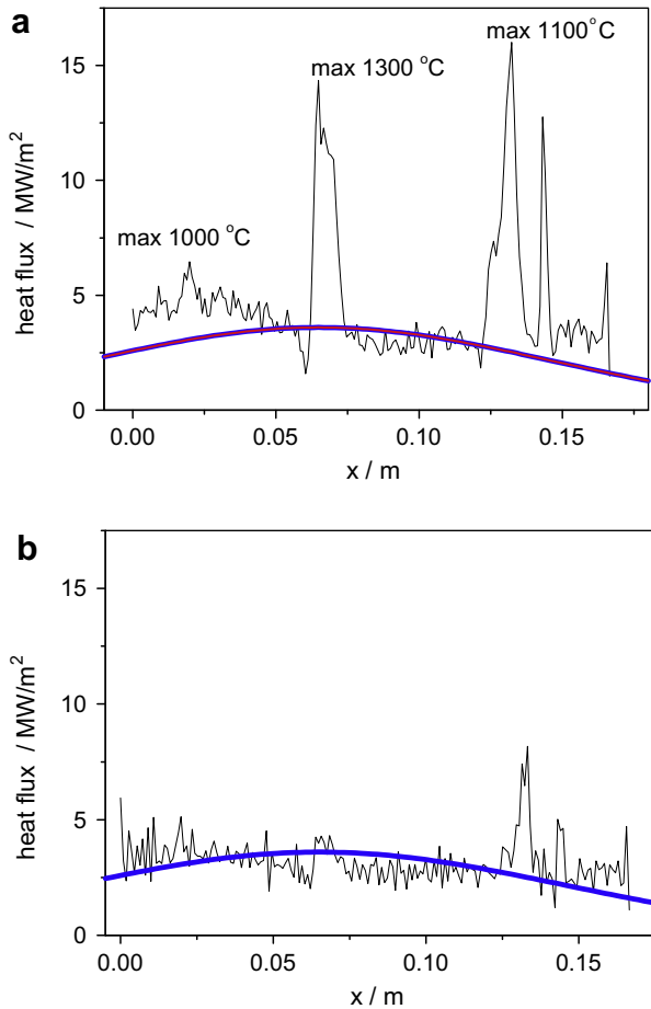
Fig. 6. Comparison of the calculated heat flux density profile about 30 ms after beginning of the heat pulse with the actual values for the first and last pulse on tile 5.
