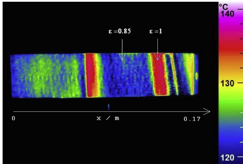
Fig. 1. Thermal image of divertor tile 5 after uniform warming indicating the apparent temperature and derived emissivity values inside and outside the stripe zones.
