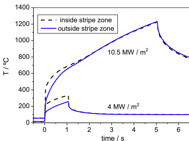
Fig. 3. Surface temperature evolution in- and outside the stripe zones of tile 13 for the two first pulses indicating the convergence of the temperatures for values beyond 700 \text{ °C} .
