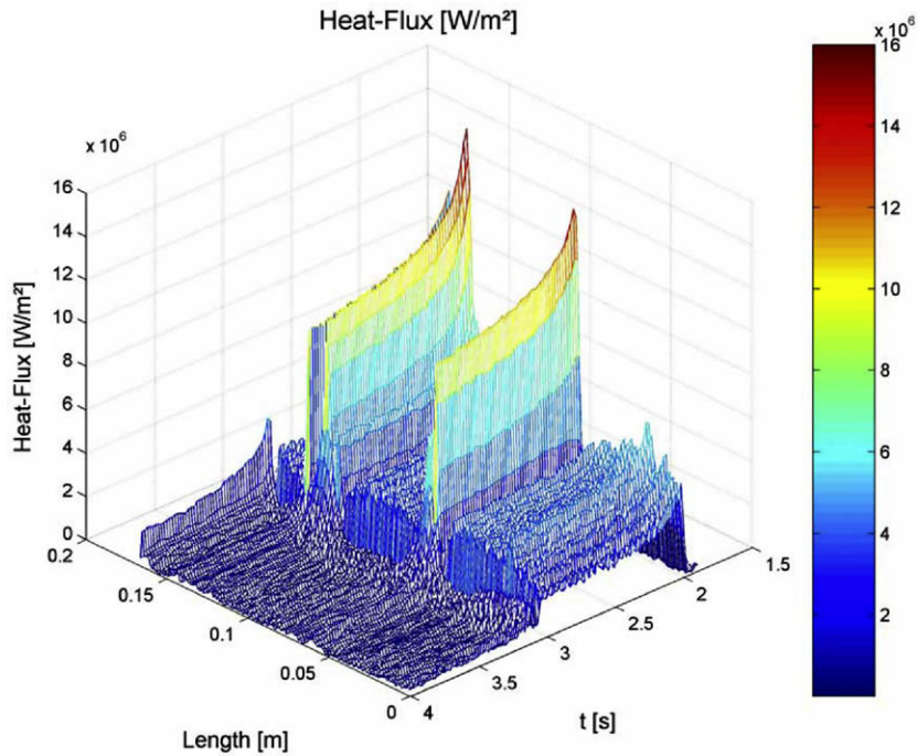
Fig. 5. Spatiotemporal heat flux densities calculated from the temporal evolution of the measured temperature distribution for the first pulse with 4 MW/m 2 on tile 5.
