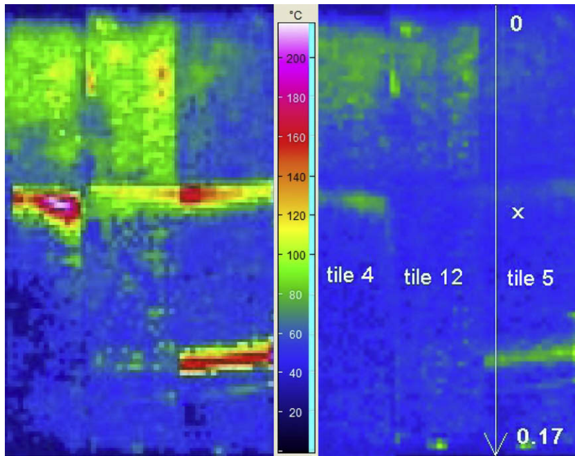
Fig. 2. Surface temperature pattern on 3 different tiles as the response of a nearly uniform heat flux about 30 ms after the beginning of the first (left side) and the last pulse (right side) with 4 \text{ MW/m}^2 . Between the first and the last pulse 2 further pulses with 10.5 \text{ MW/m}^2 with durations up to 5 s were performed.
